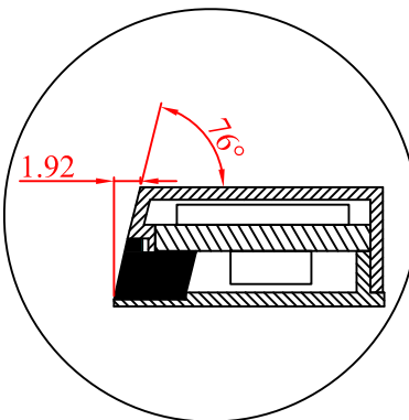
Detail A 6:1
