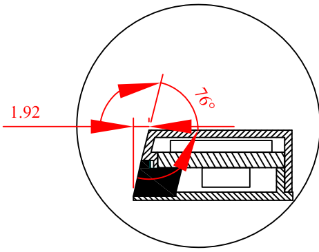
Detail A 5:1
