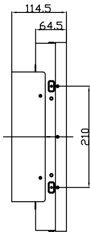
SIDE MOUNT, VERTICAL
