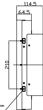
SIDE MOUNT, VERTICAL
