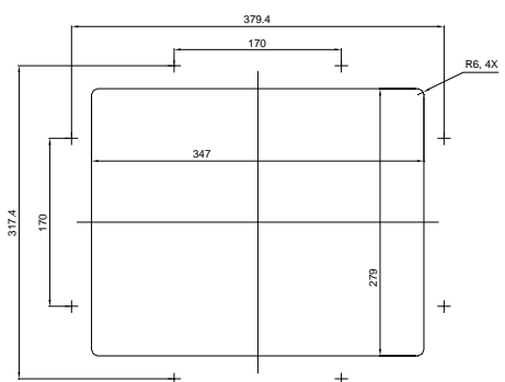
RECOMMEND CUSTOMER PANEL CUT-OUT
