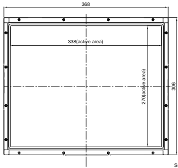
RECOMMEND CUSTOMER PANEL CUT-OUT
