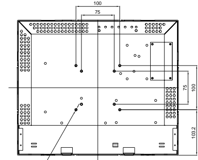
8-Ø7 M4 THREAD VESA MOUNT MAX. SCREW DEPTH 11±0.2mm
