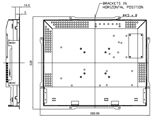
MOUNTING BRACKET ADJUSTMENT RANGE REAR MOUNT WITH BRACKETS HORIZONTAL OR VERTICAL
