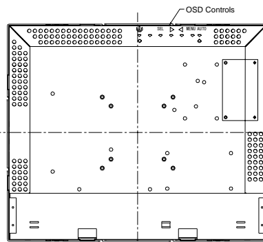
VESA MOUNT
